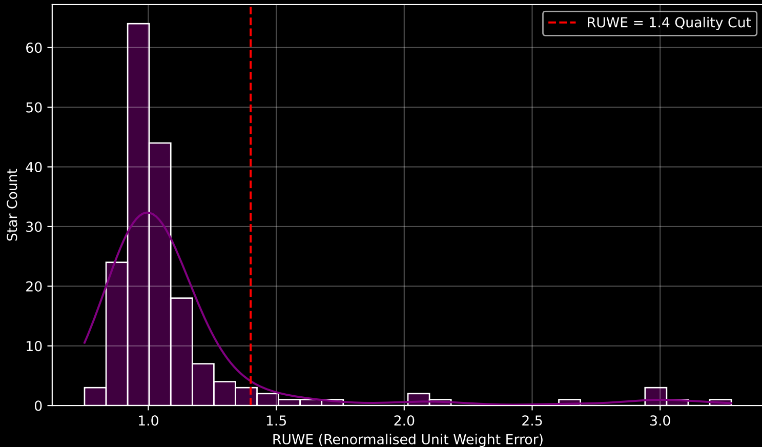
GAPOGEE DR17 Field [186+48] RUWE Distribution (n= 181)
