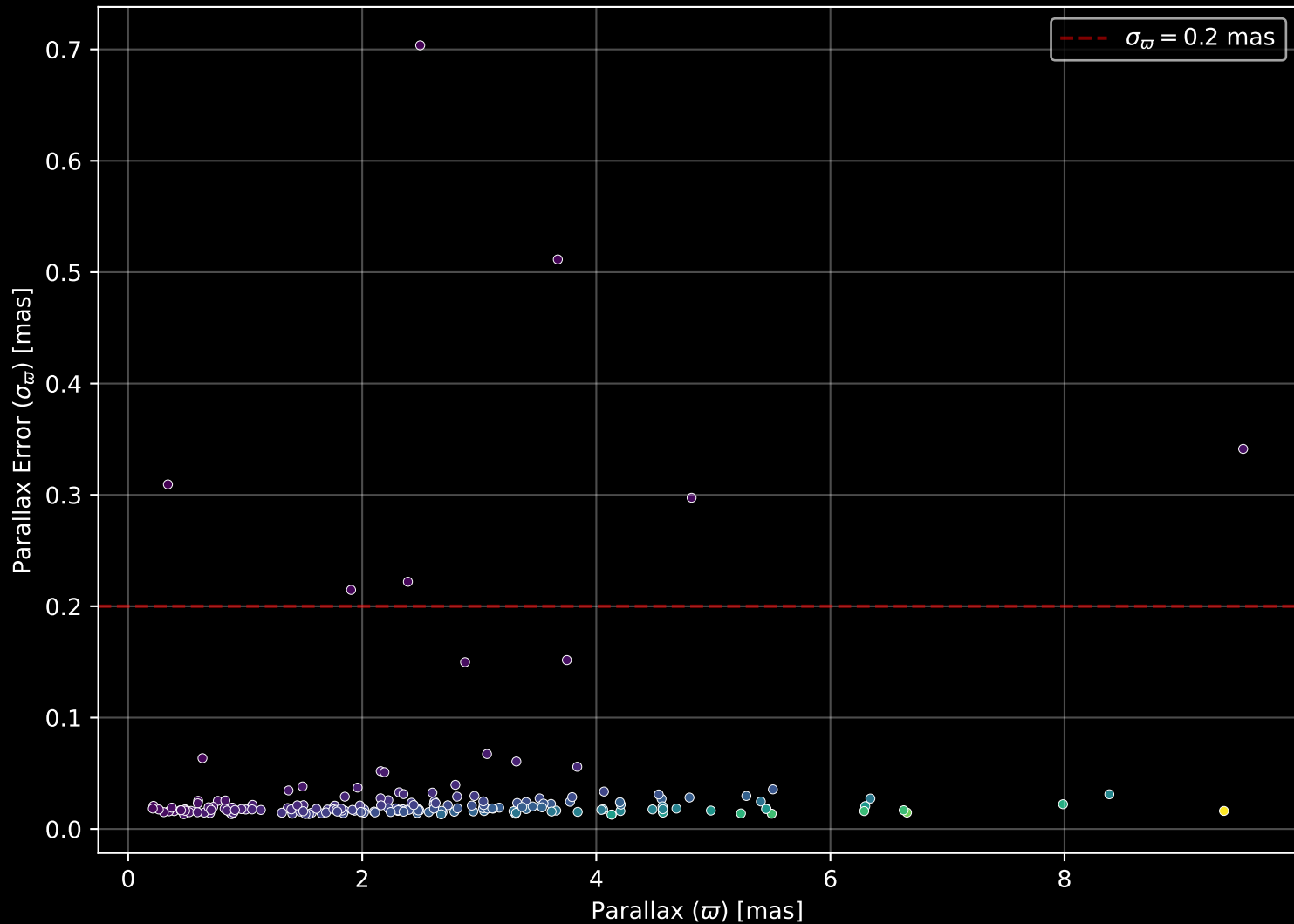
APOGEE DR17 Field: [186+48] Parallax Quality (n= 190)
