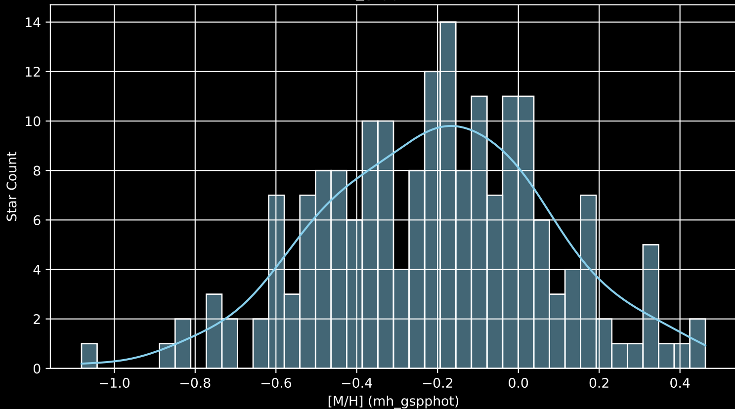
APOGEE DR17 Field: [186+48 [M/H] (mh_gspphot) (n= 189)
