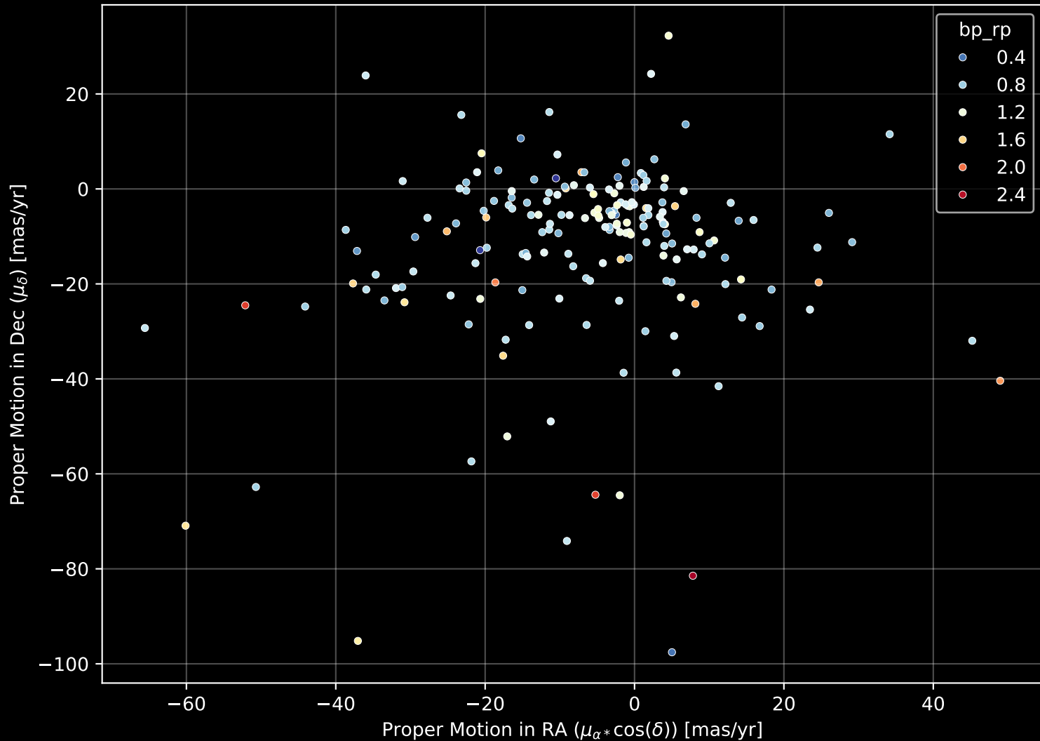
APOGEE DR17 Field: [186+48] Proper Motion Diagram (n= 190)
