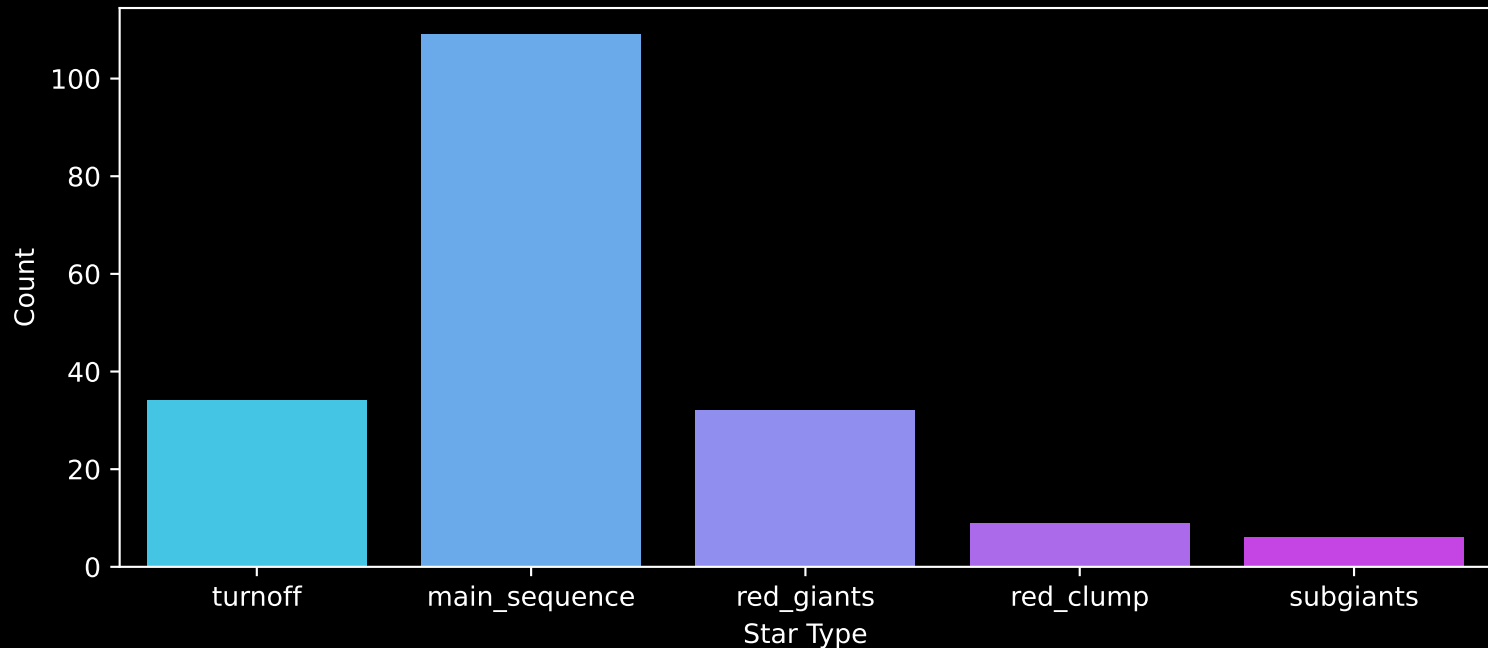
APOGEE DR17 Field: [186+48] Count plot of Star Type
